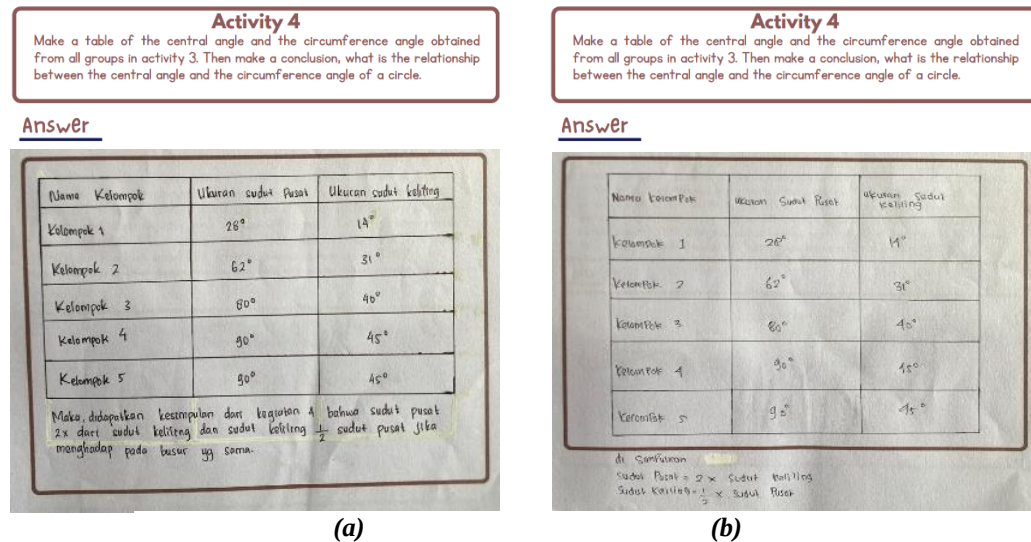
(a) (b) Figure 4. Table of Central Angle and Circumference Angle Measurements and Their Relationship
